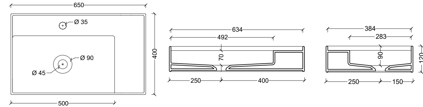
31120101 Lavabo HIDE STADIUM
