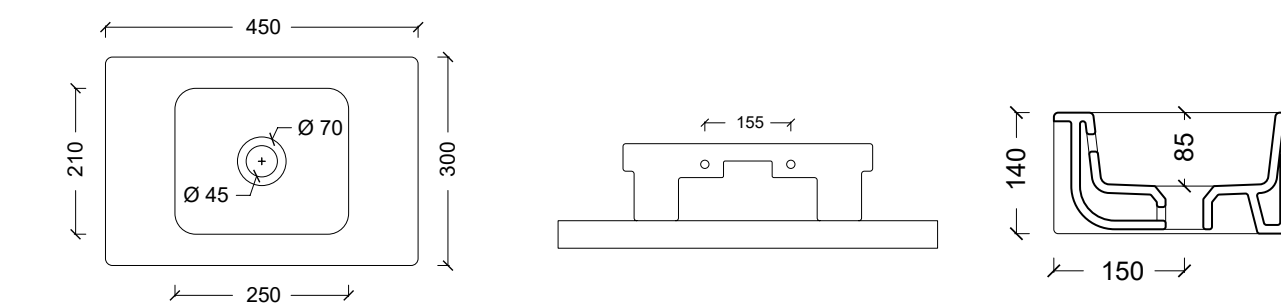
20150801 Lavabo LOGIC 42 X 22
