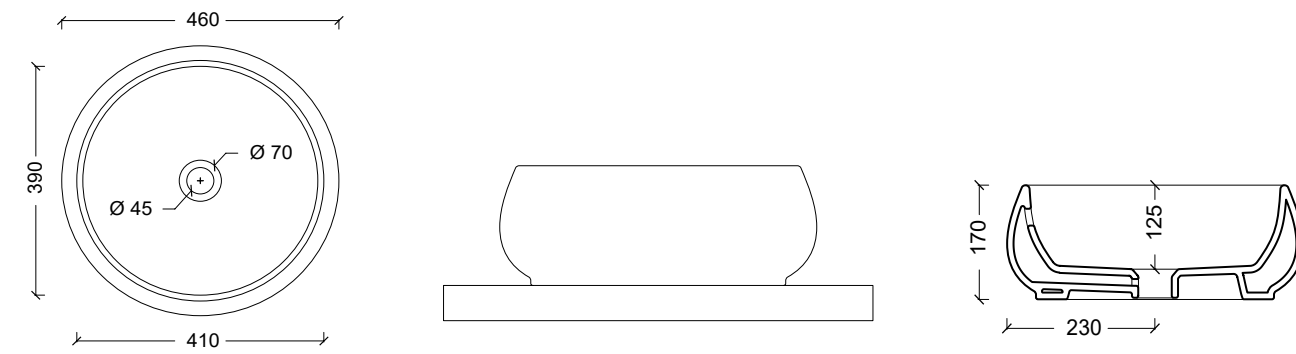
24100301 Lavabo TULIP SMALL
