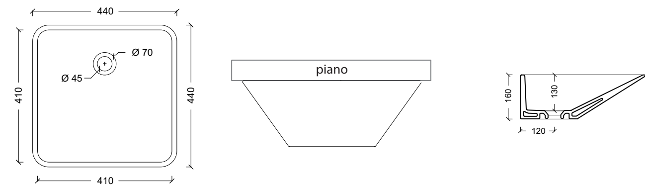
26150101 Lavabo EDGE 44X44 UNDERCOUNTER
