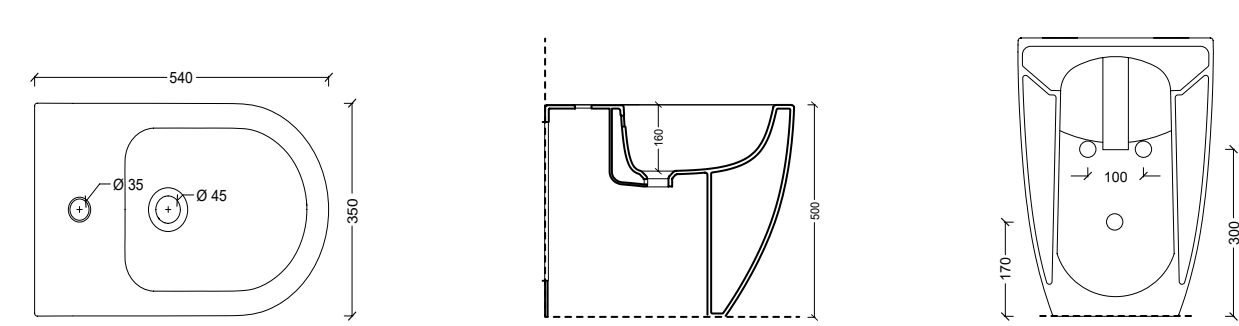
22280101 Bidet a terra H 50 FORM SQUARE
