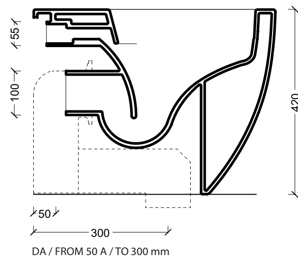
Vaso FORM SQUARE TERRA TRASLATO
