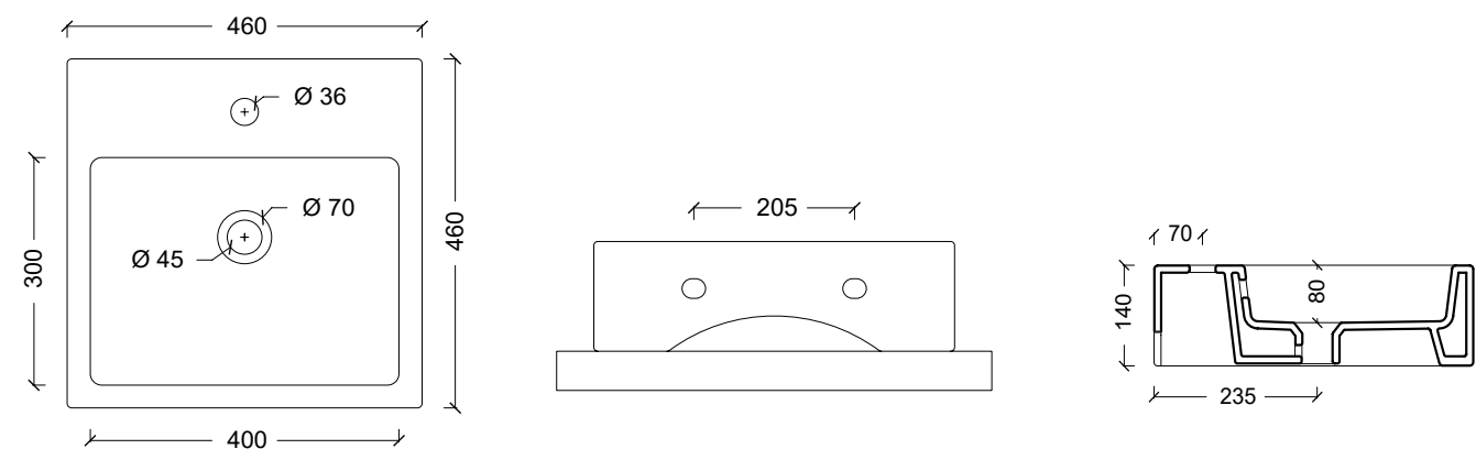
20160101 Lavabo ICE 46X46
