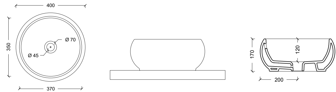
24100301 Lavabo TULIP SMALL
