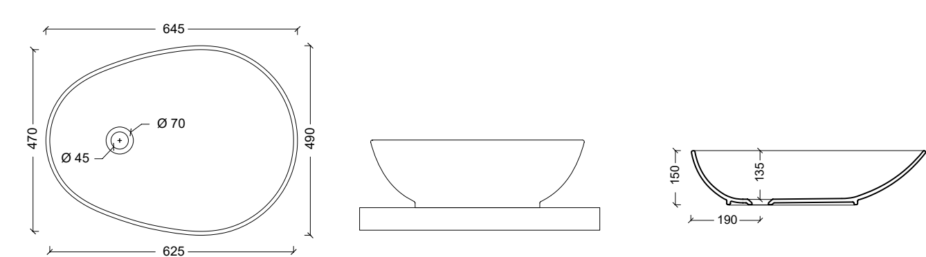
29130301 Lavabo JOKER SPOON
