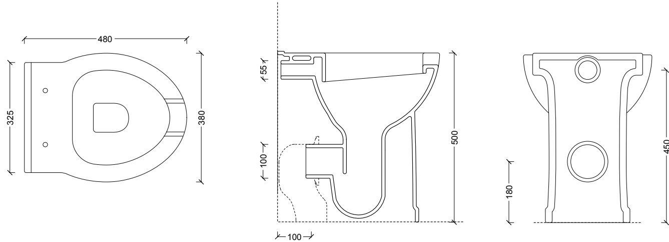
30190101 VASO SHORT A TERRA H50 OPEN
