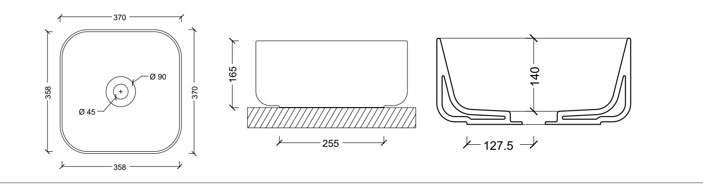
32190101 Lavabo UNICA 50x37
