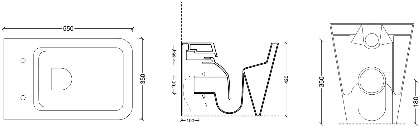
31190101 Vaso a terra HIDE SQUARE
