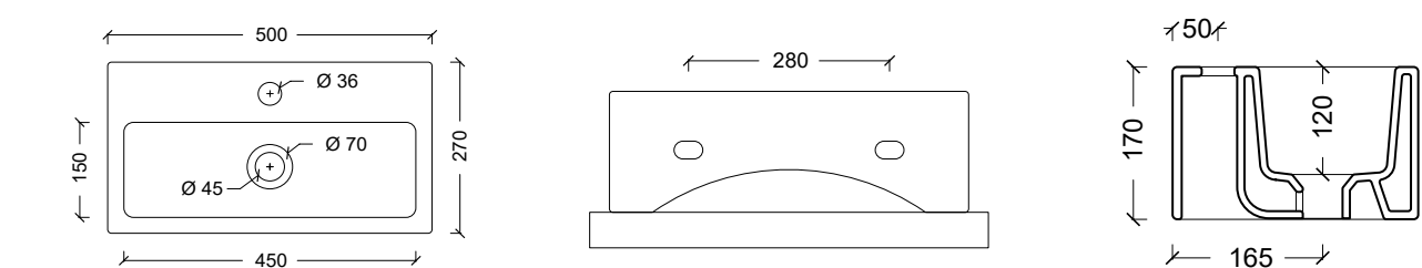
20100101 Lavabo ICE 40 X 20
