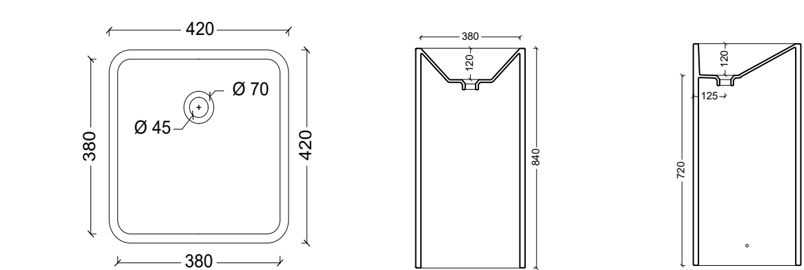
29200301 Lavabo JOKER TRAY
