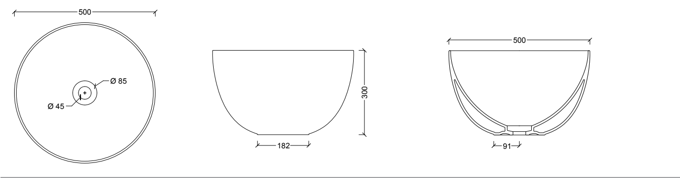
32140101 Lavabo UNICA SQUARE
