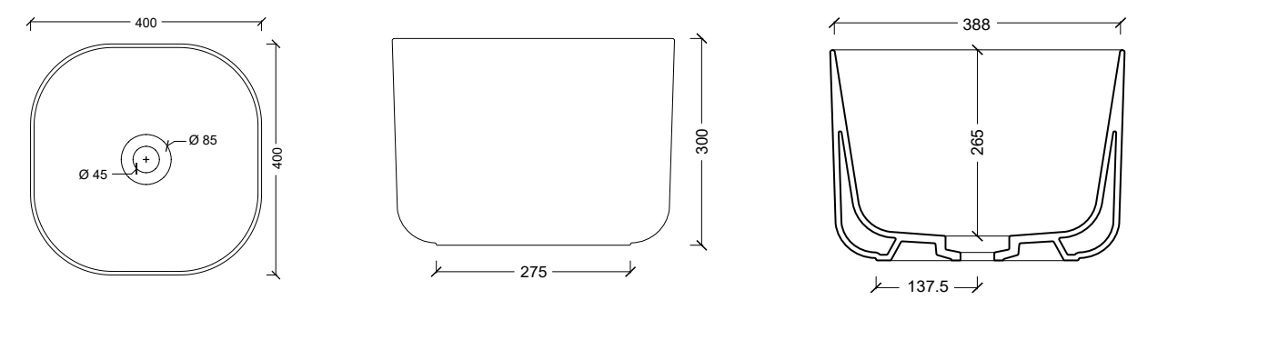
32150101 Lavabo UNICA RECTANGULAR
