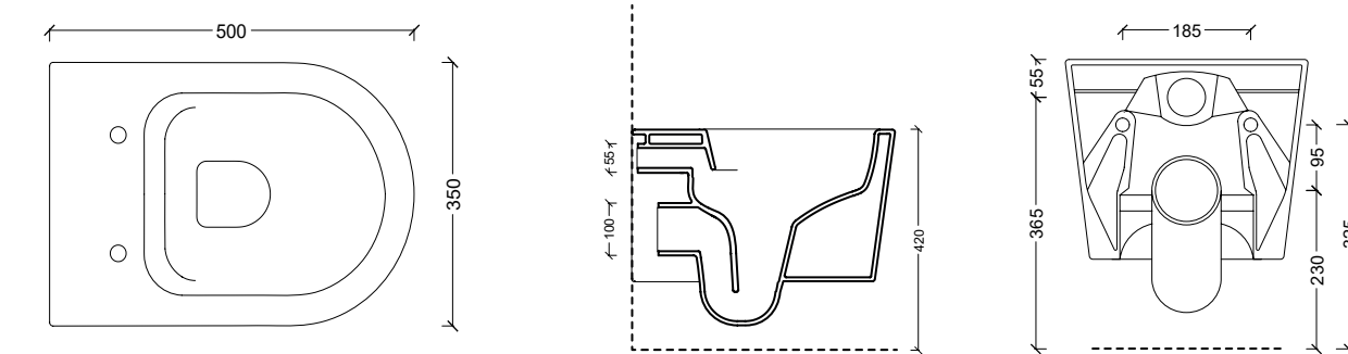
22300101RL Vaso sospeso FORM SQUARE
