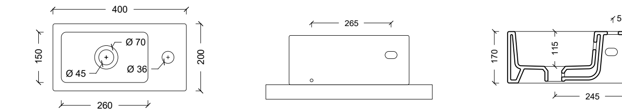
20170501 Lavabo ICE 52 X 26
