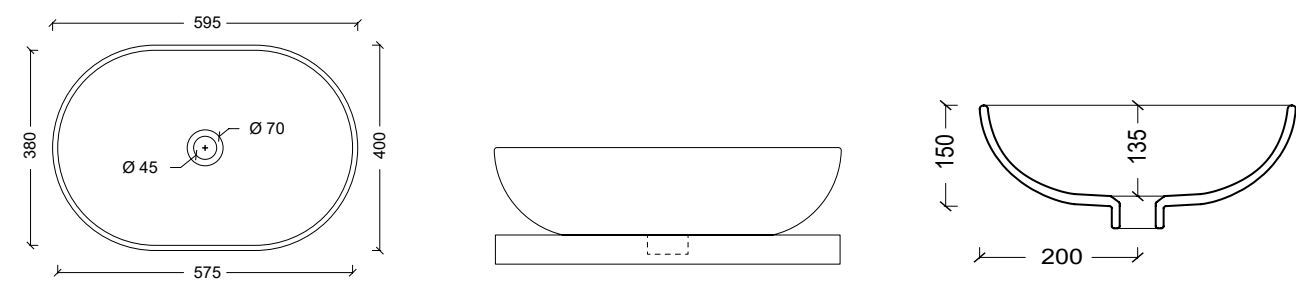
29170101 Lavabo JOKER POT
