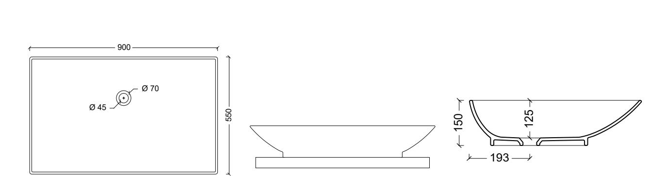
29200301 Lavabo JOKER TRAY
