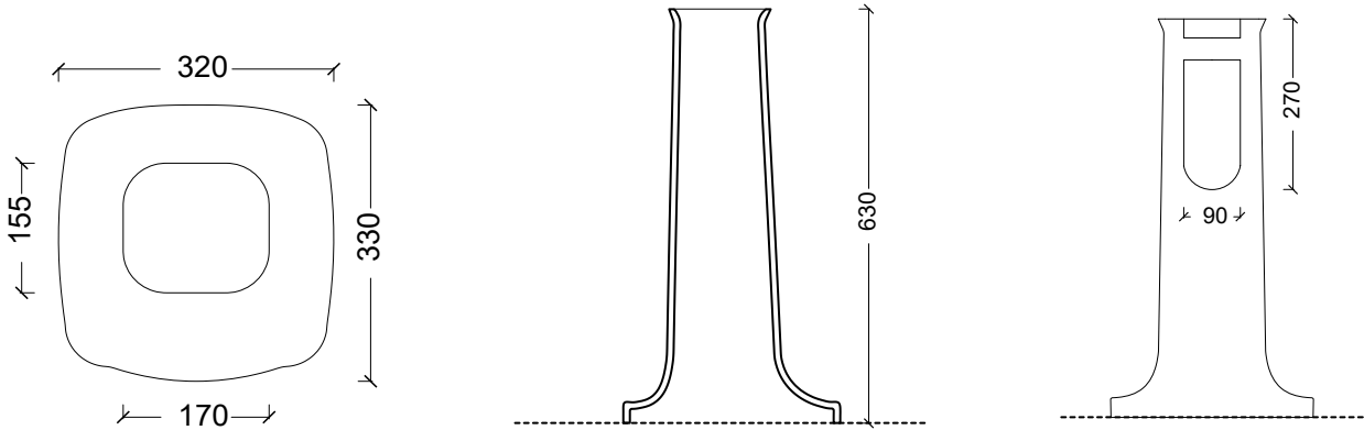
28240101 Colonna LAVABO BOHEME 70
