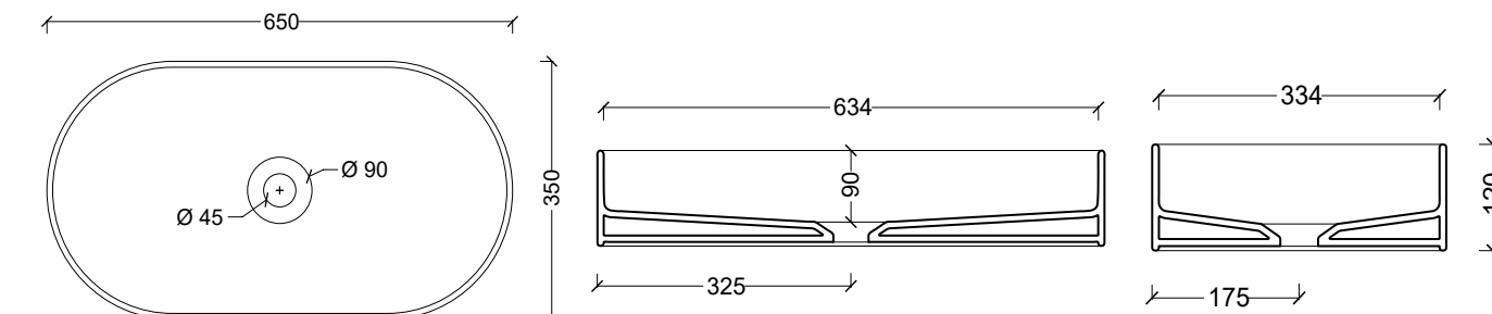
31120101 Lavabo HIDE STADIUM
