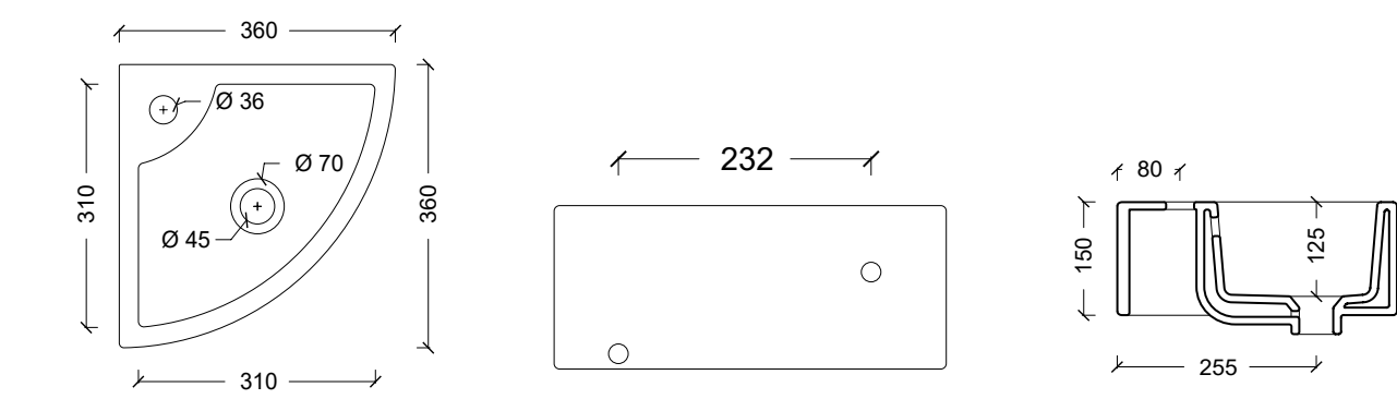
21100801 Lavabo LOGIC 60 X 35
