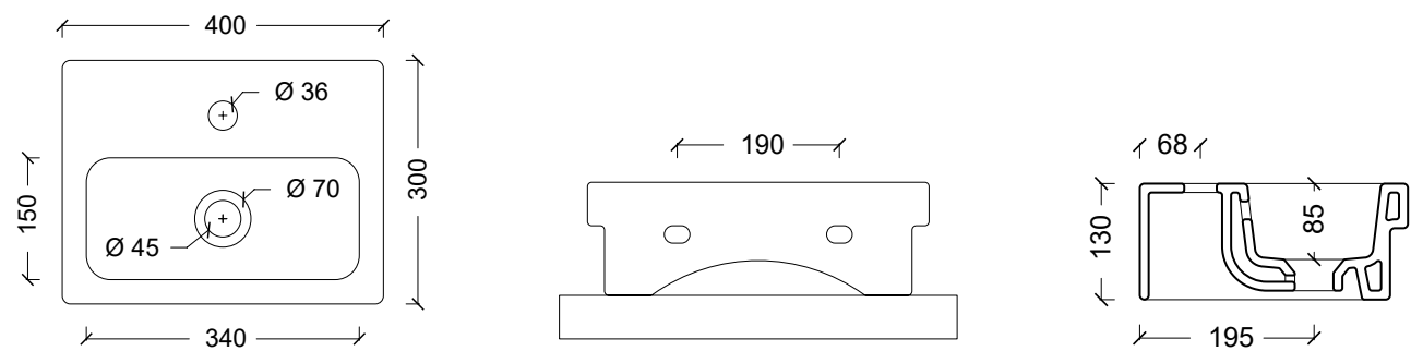
21160801 Lavabo LOGIC 35 X 35
